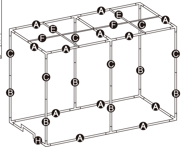
Steel Tube Frame with steel corner
